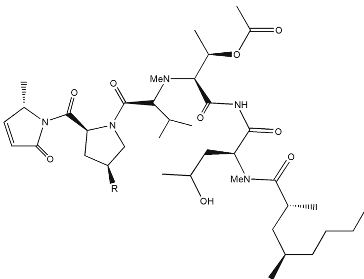
5, R = OH 6, R = H
