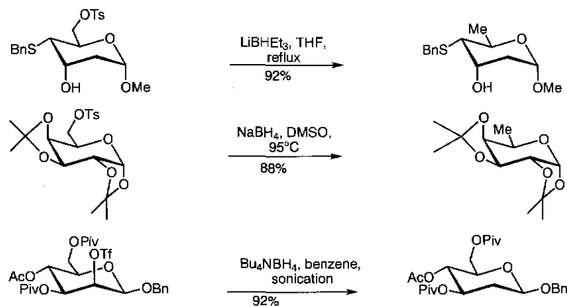
Scheme 3.8 Deoxygenation of saccharides.
