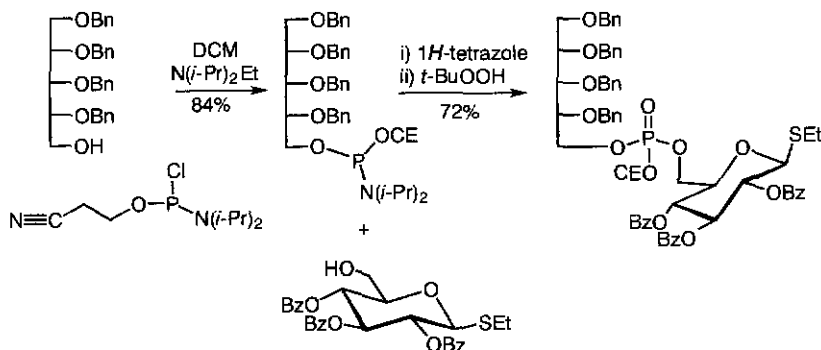
Scheme 3.18 Phosphorylation by phosphite method.
