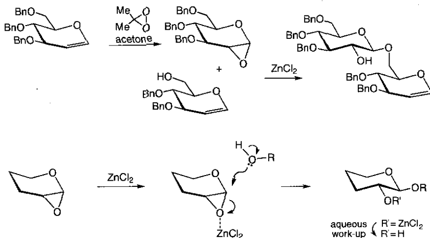
Scheme 4.8 (Continued).
