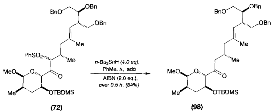
Scheme 17.25.
