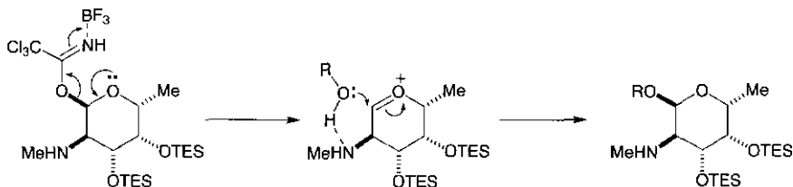
Scheme 8.13.
