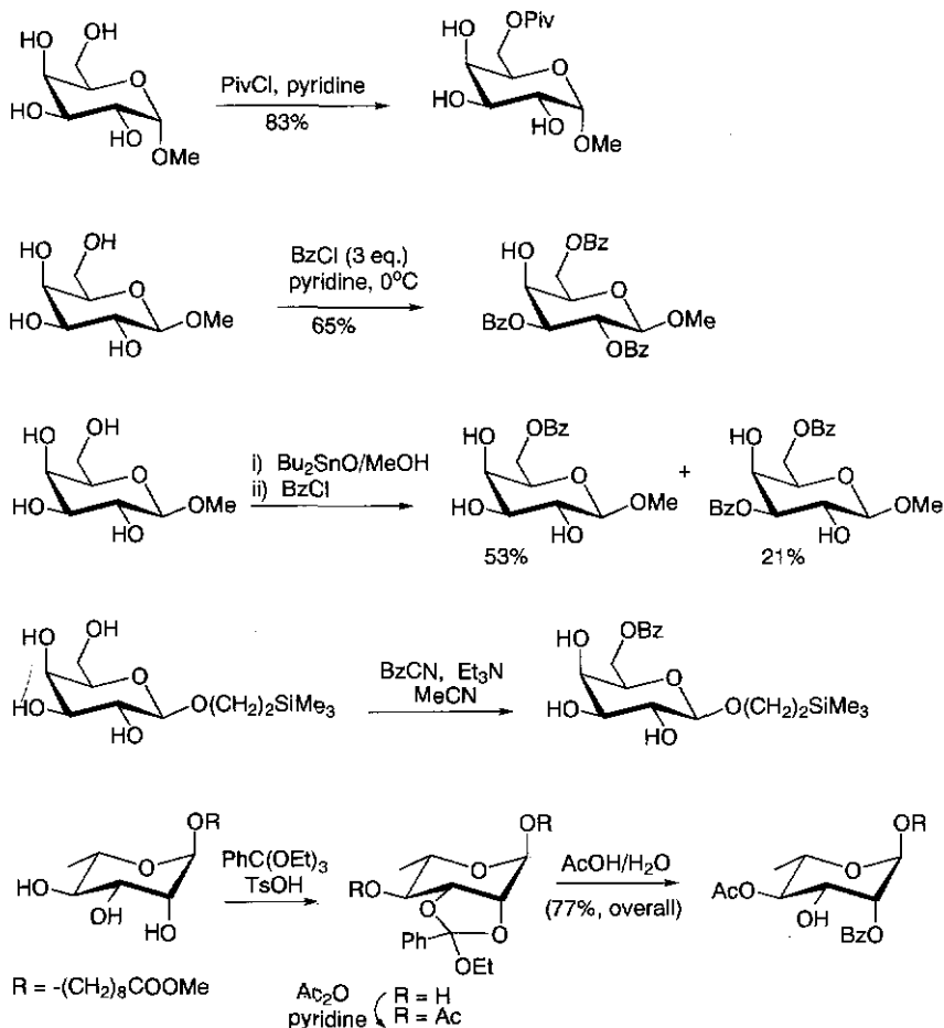
Scheme 2.13 Regioselective acylations.
