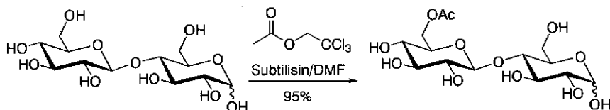
Scheme 2.14 Regioselective acylation using lipases.
