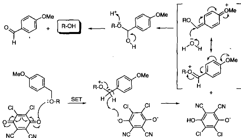
Scheme 2.5 Mechanism of cleavage of p -methoxybenzyl ethers with 2,3-dichloro-5,6-dicyano-1,4-benzoquinone. Note: SET = single-electron transfer.
