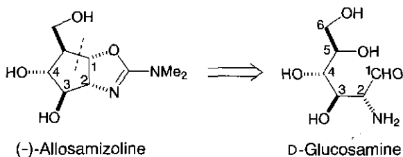
Scheme 11.1 The conceptual conversion of (-)-allosamizoline to D-glucosamine.
