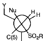
Figure 3.1 Unfavourable steric and electronic interactions in nucleophilic displacements of sulfonates. Note: Ts=transition state.
