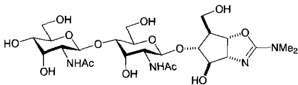
Figure 11.1 (-)-Allosamidin.
