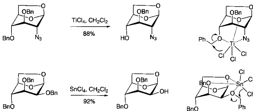
Scheme 2.3 Regioselective debenzylations.
