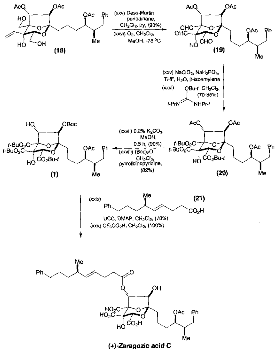
Scheme 7.4 (Continued).
