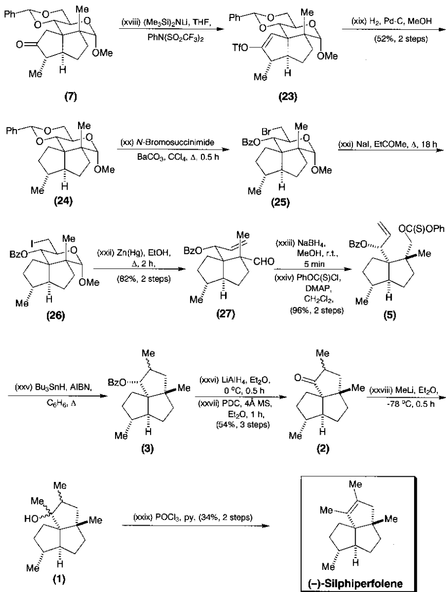
Scheme 10.5 (Continued).
