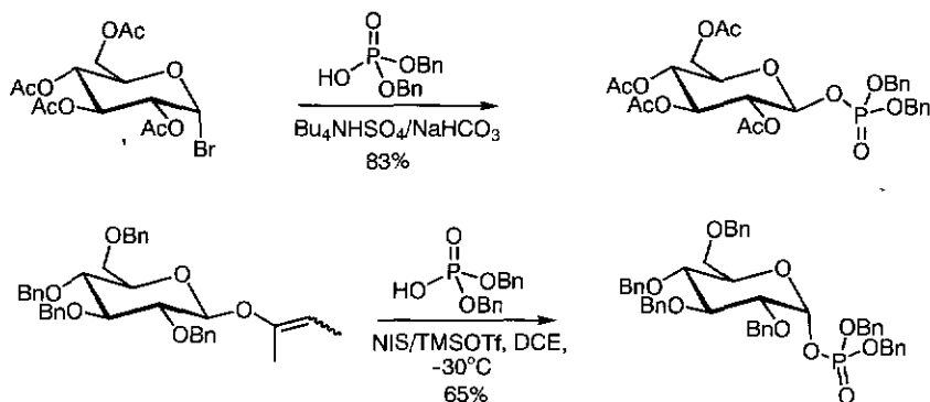
Scheme 3.20 Anomeric phosphorylation.
