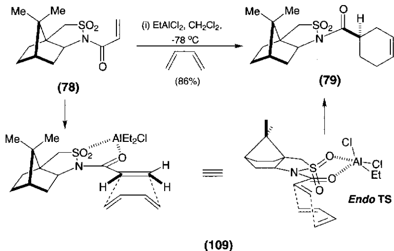
Scheme 17.29.
