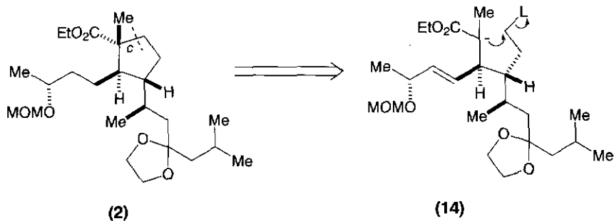
Scheme 12.4.
