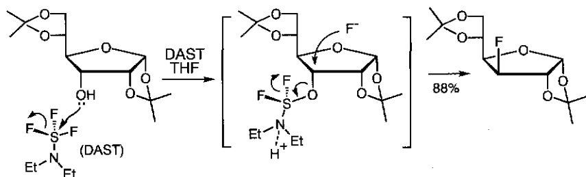
Scheme 3.2 (Continued).
