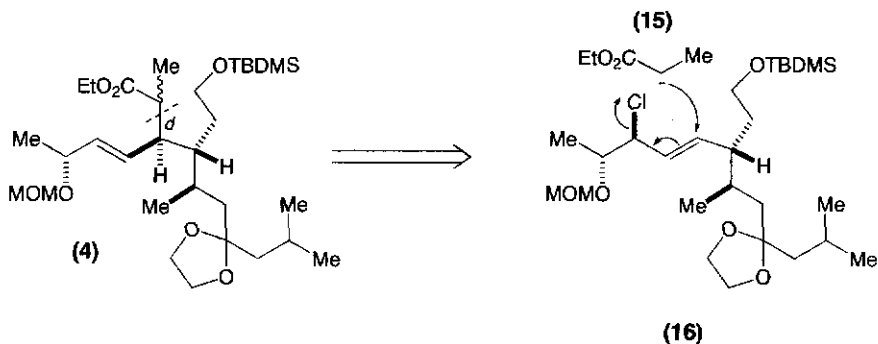
Scheme 12.5.
