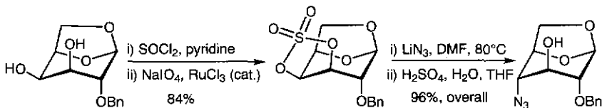
Scheme 3.10 (Continued).
