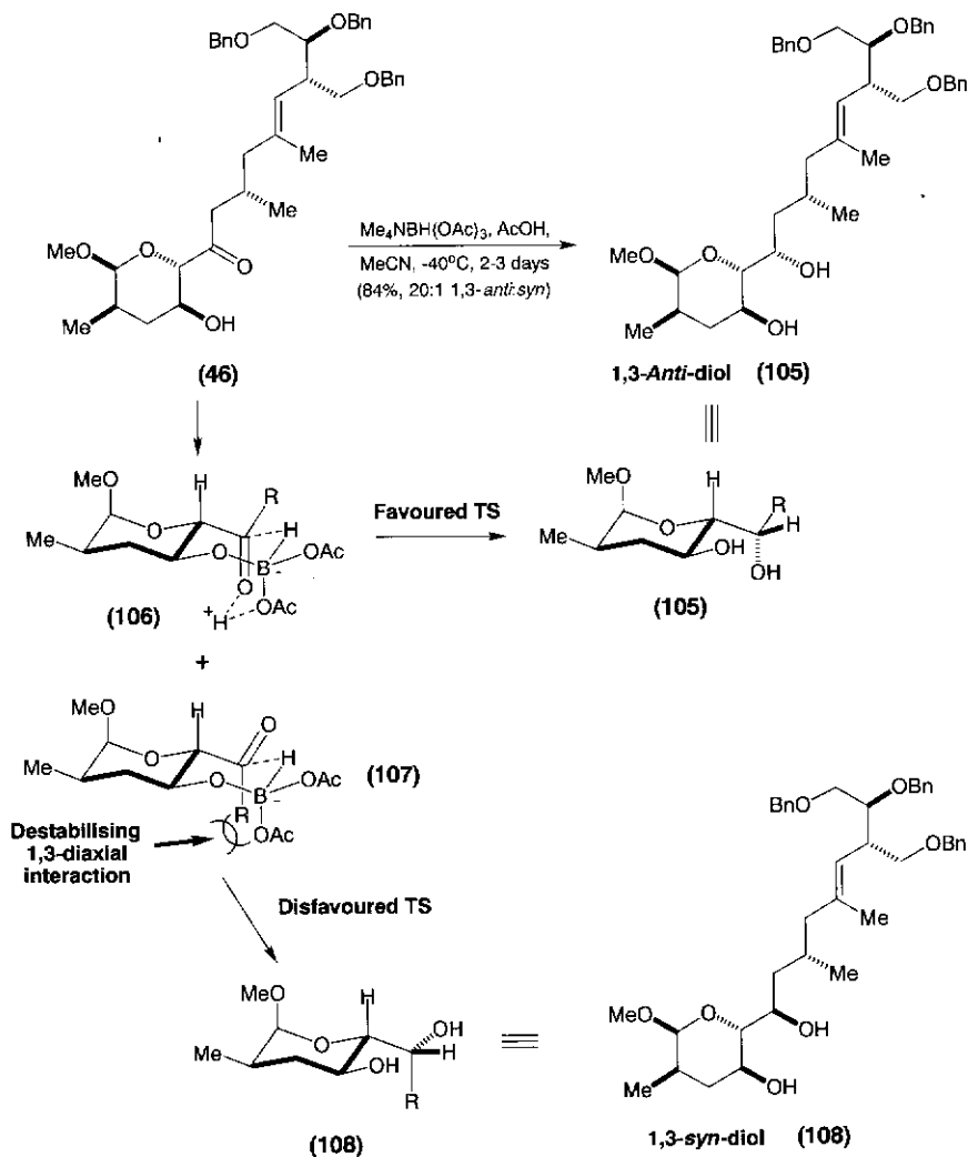
Scheme 17.28.
