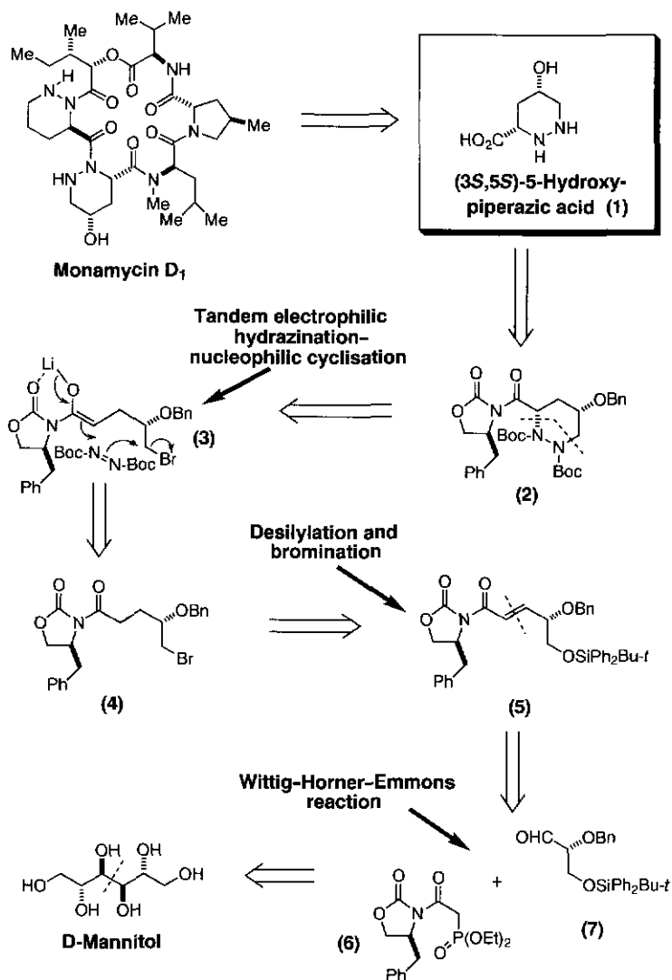
Scheme 18.1 The Hale retrosynthetic analysis of (3 S ,5 S )-5-hydroxypiperazic acid.
