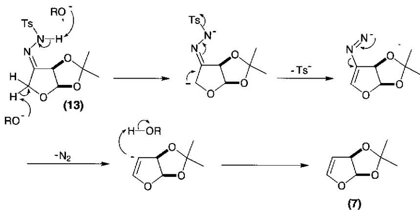
Scheme 6.6.
