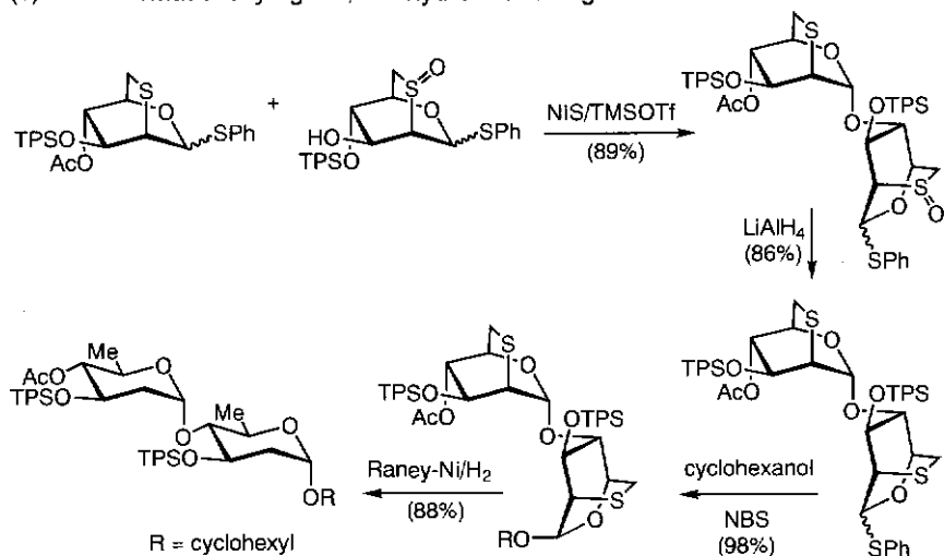
Scheme 4.13 (Continued).
