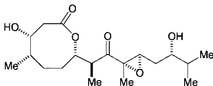
Figure 13.1 (-)-Octalactin A.
