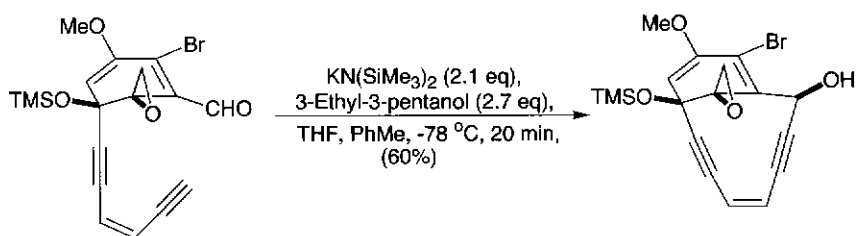
Scheme 8.5 Acetylenic anion ring-closure in Danishefsky's calicheamicinone synthesis.
