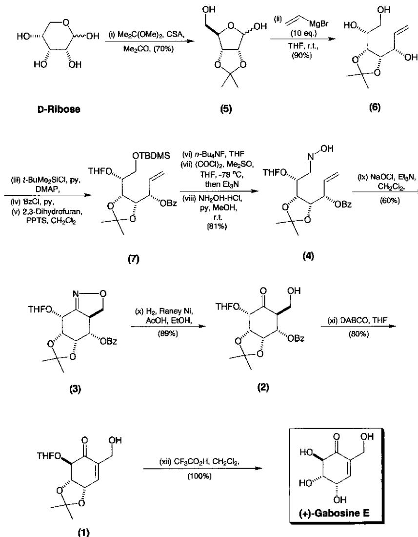
Scheme 15.3 Lygo's synthesis of (+)-gabosine E.
