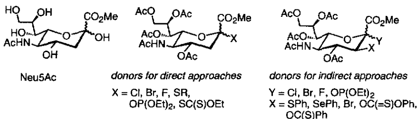
Scheme 4.12 Glycosylation of N -acetyl-neuraminic acid (Neu5Ac) by direct and indirect approaches.
