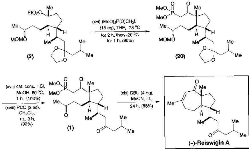
Scheme 12.6 (Continued).
