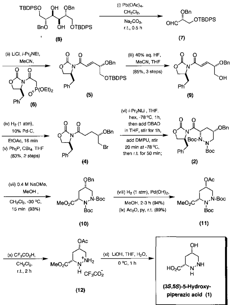
Scheme 18.2 Hale's enantiospecific synthesis of (3 S ,5 S )-5-hydroxypiperazine acid.
