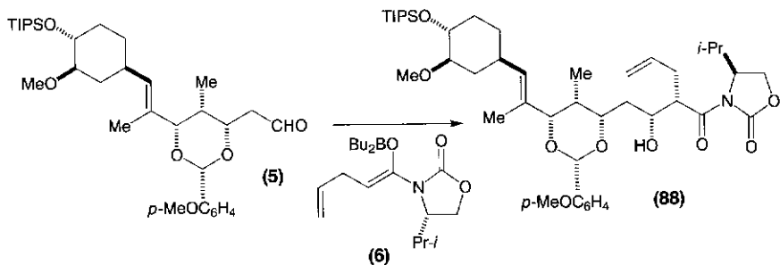
Scheme 17.21.
