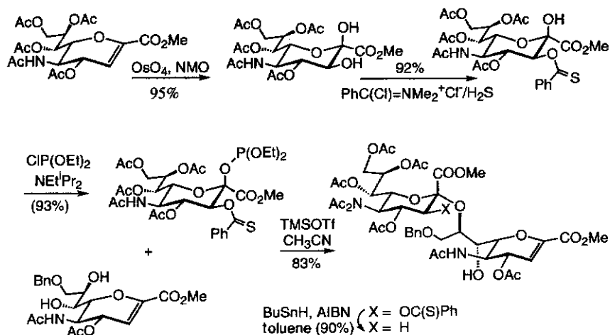
Scheme 4.12 (Continued).
