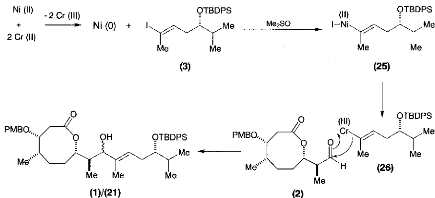
Scheme 13.6.
