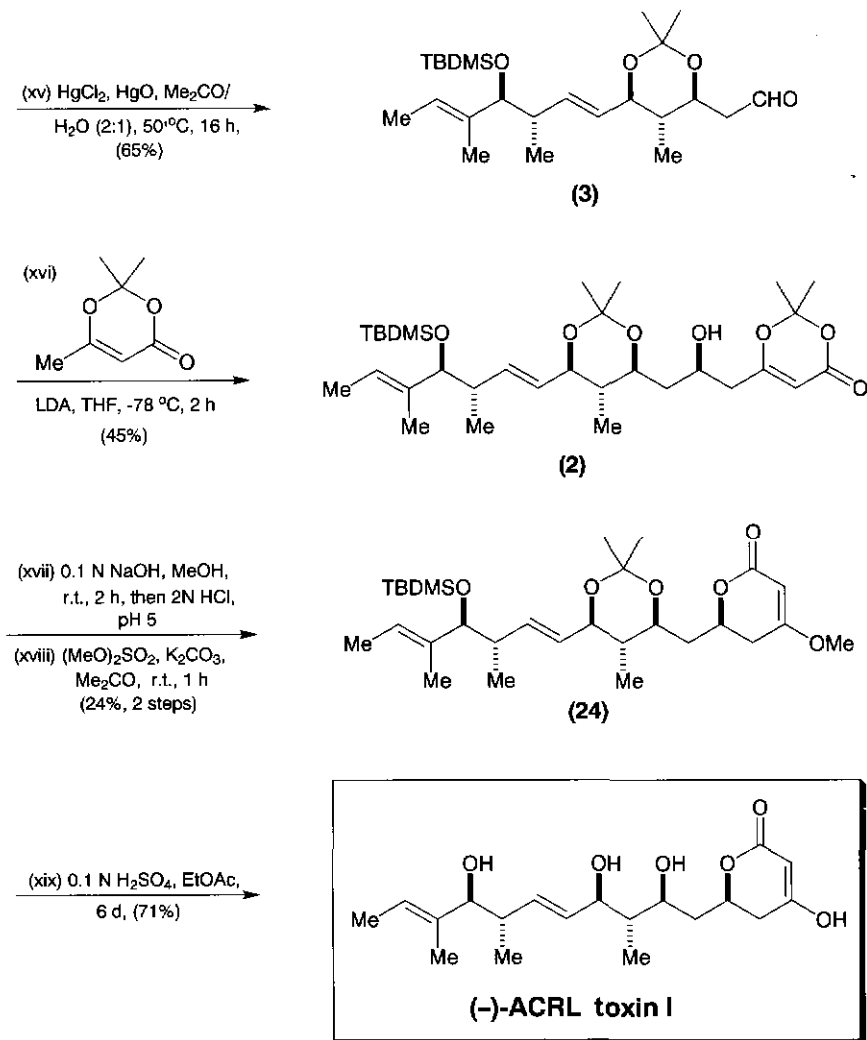
Scheme 14.4 (Continued).
