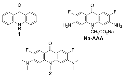
Figure 1. Structures of acridone ( 1 ), acridone acetic acid, sodium salt ( Na-AAA ), and fluoros acridone ( 2 ).
